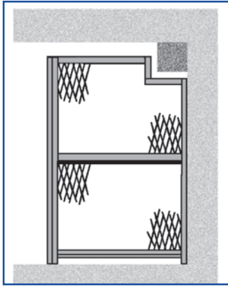
SHOWING CUT OUT (WITH REPAIR ANGLES) TO ALLOW FOR INTERFERING DUCT.
