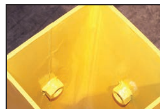
Grade 5 hex nuts are welded inside posts providing maximum bolt grip for superior installation
