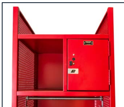
OPTIONAL SECURITY BOX USES TWO HEAVY-DUTY 13 GAUGE 7-KNUCKLE 3-1/2" HINGES AND A FINGER PULL PADLOCK HASP
